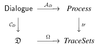
Figure 3: Dialogue compiler correctness.
